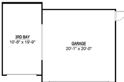
OPTIONAL 3RD BAY GARAGE
