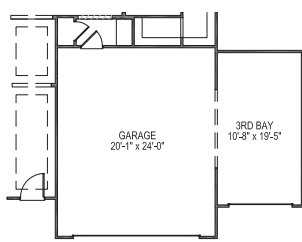
OPTIONAL 3RD BAY GARAGE
