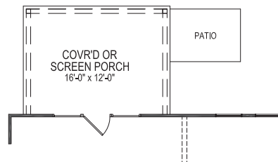
OPTIONAL COVERED OR SCREENED PORCH
